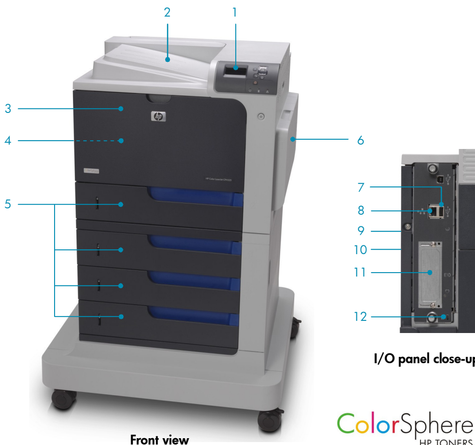
HP Color LaserJet Enterprise CP4525xh Printer shown
